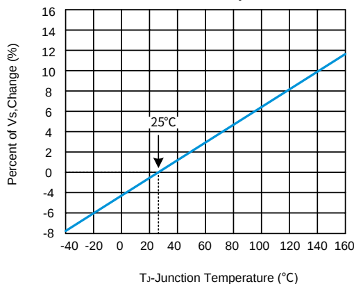
Fig.2 Normalized Vs Change versus Junction Temperature
