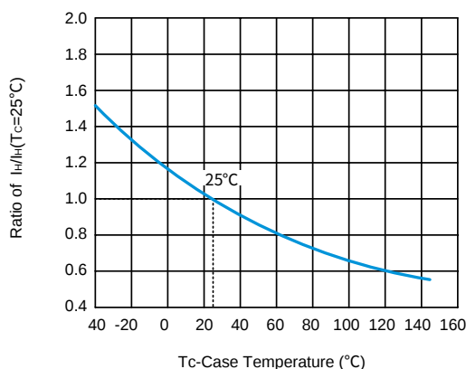
Fig.3 Normalized DC Holding Current versus Case Temperature
